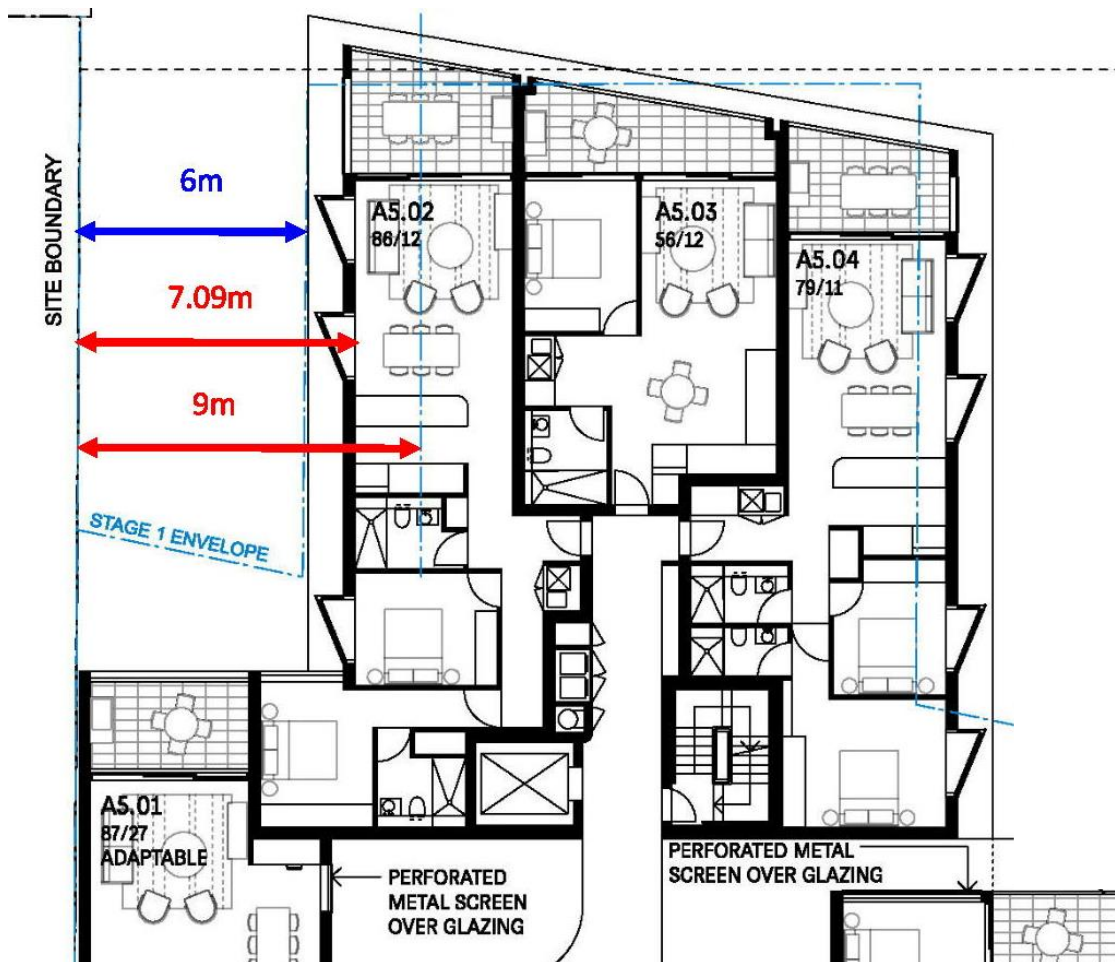
Figure 29: Building Separation - Building A and south-western property boundary adjoining Petbarn
