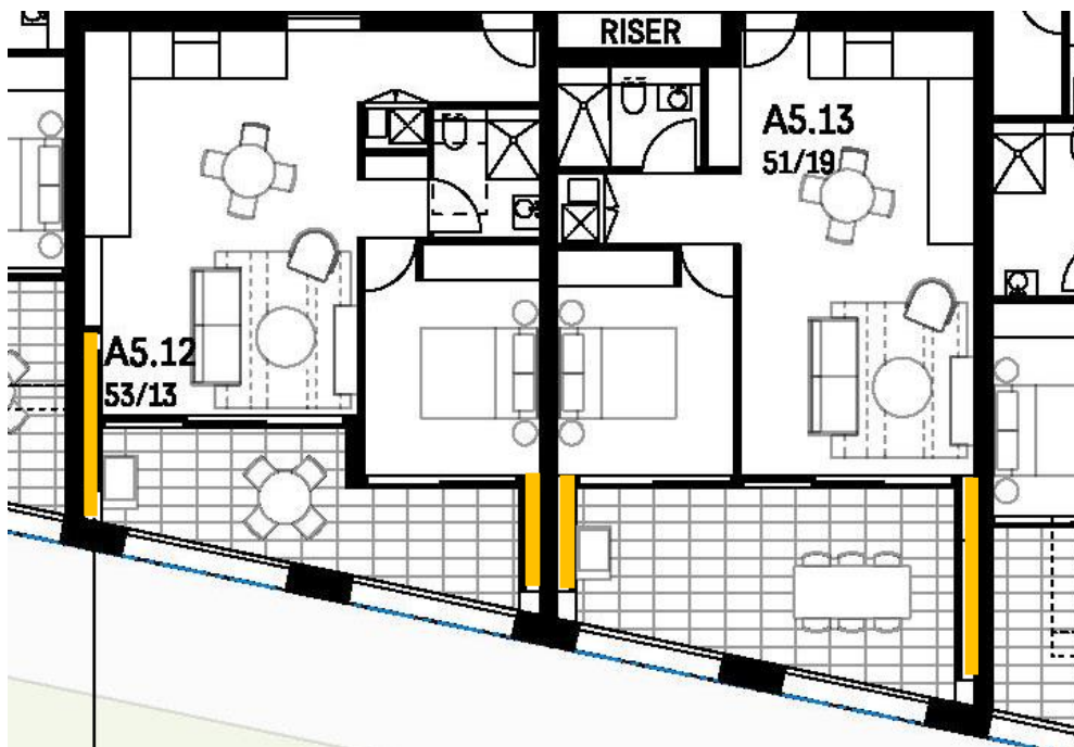
Figure 35: Integrated vertical plenums to McEvoy Street apartments shown in yellow
