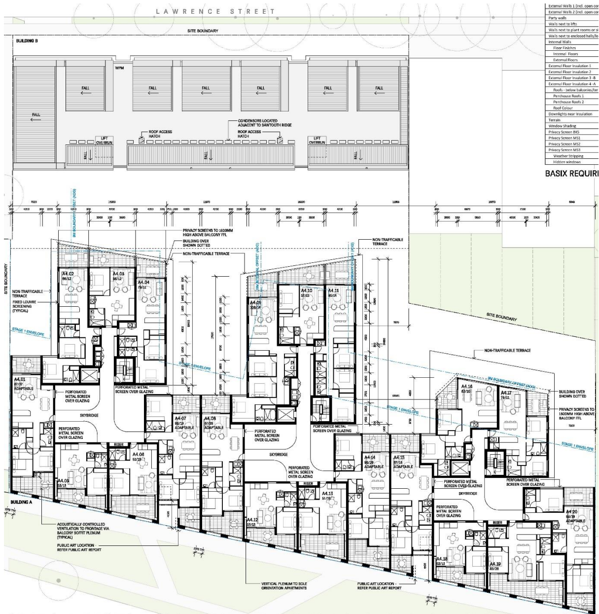
Figure 21: Level 4 Floor Plan
