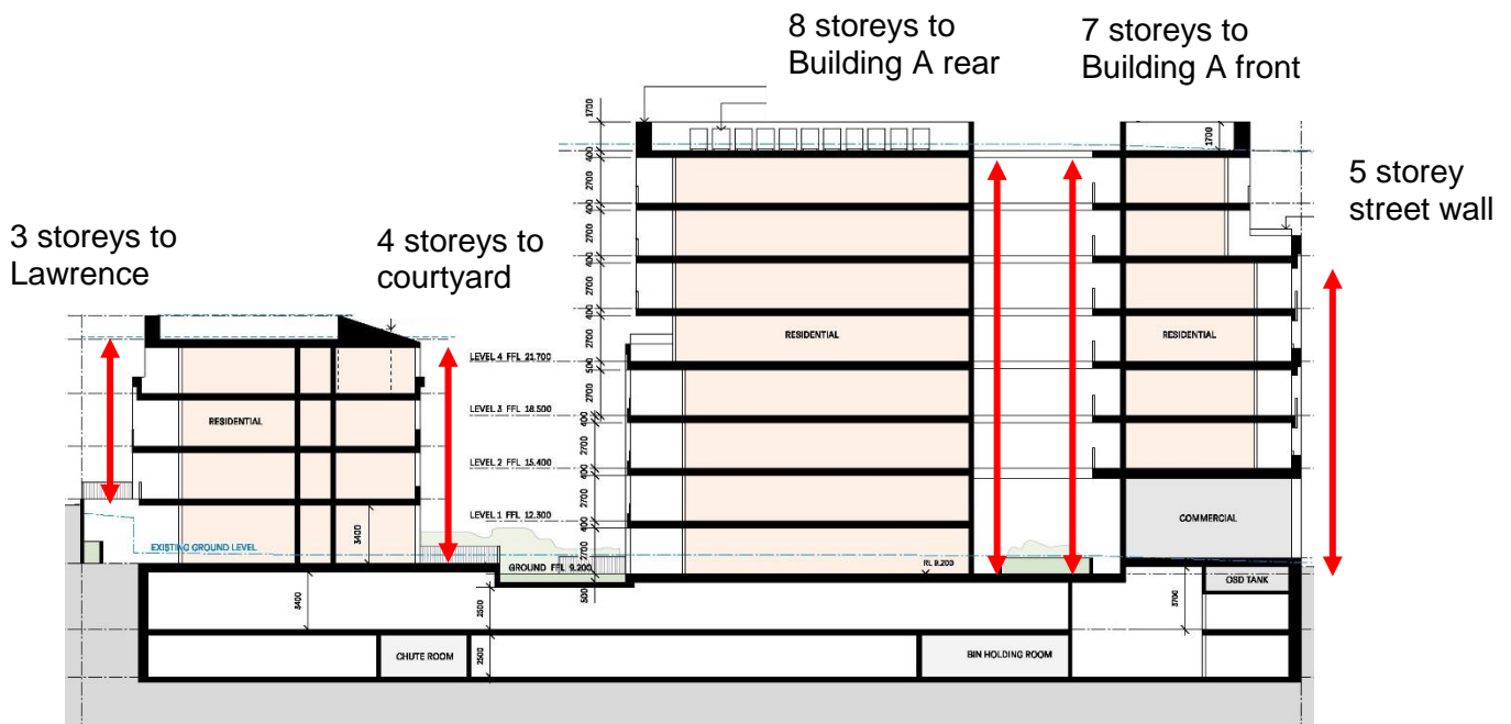
Figure 28: Height in storeys non-compliance, Buildings A and B
