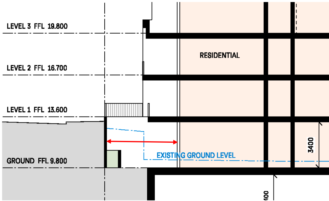
Figure 26: Minimum 5m setback to glass line
