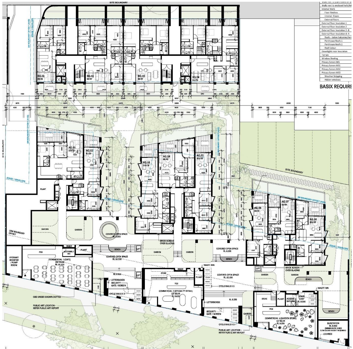
Figure 19: Ground Floor Plan
